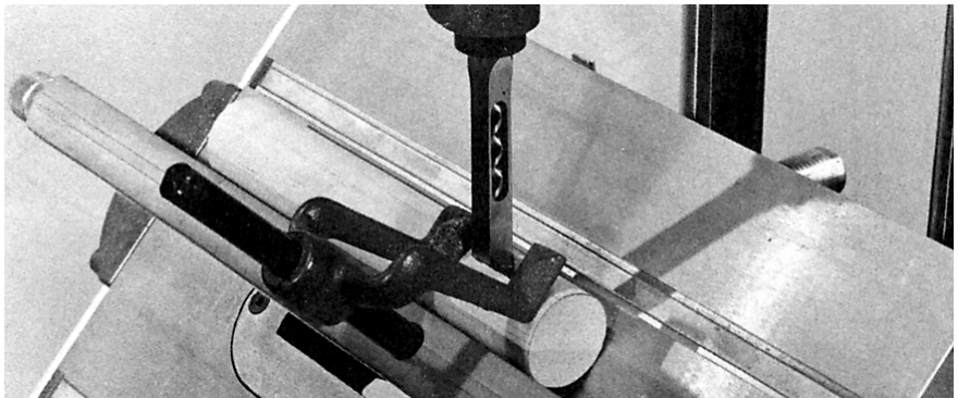
Figure 8-7. The fence/table V-block arrangement can be used to hold round workpieces for mortising. Be sure to mark the workpiece so the cuts will begin and end on the same line.
